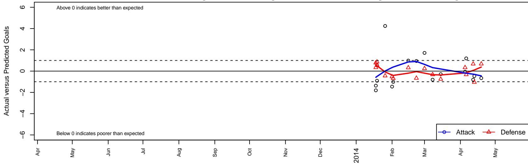
Crossfire Oregon Black East B97 Dots are actual minus expected GF (blue circles) and GA (red triangles). Blue line is smoothed change in attack strength. Red is smoothed change in defense strength.
